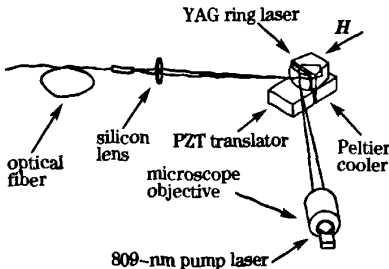
图 8 压电效应调谐激光器实验装置 Fig. 8 Schematic of the piezo-electric tuning laser
