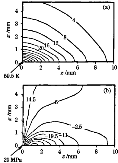
图1 端面抽运晶体中的温度(a)和应力(b)分布 Fig. 1 Temperature (a) and stress (b) distributions for the conventional crystal
