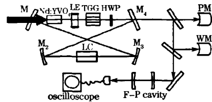
图 10 宽带电光调谐激光器实验装置 Fig. 10 Broadband electro-optic tuning laser
